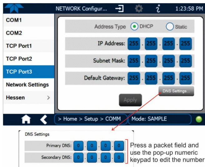
Figure 2-47. Communications Configuration, Network Settings
