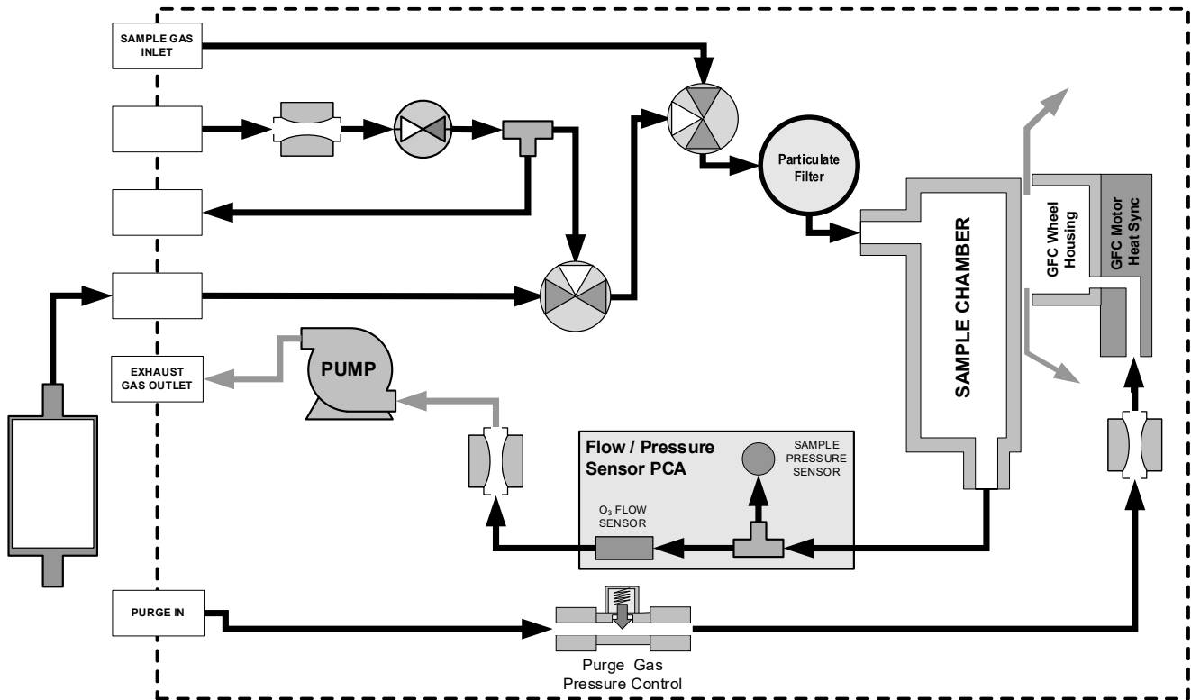
Figure 2-17. Pneumatic Flow with Ambient Zero/Pressurized Span Valves Option
