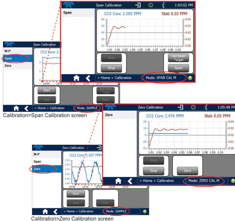
Figure 4-2. Zero and Span Calibration Screens
