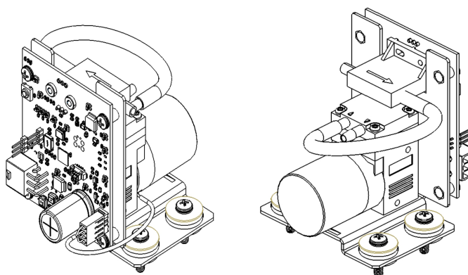
Figure 5-10. STD PID Controlled Pump
