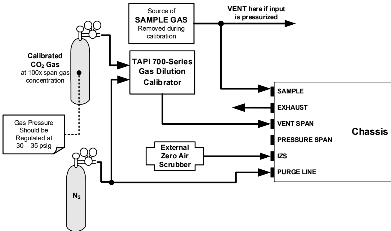
Figure 2-14. Example of Pneumatic Set up for Multipoint Calibration
